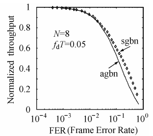
图7 GBN理论与仿真结果比较 Fig.7 Comparison of GBN simulation results and analytical performances
