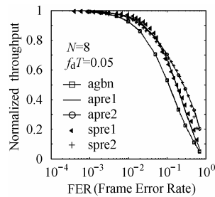
图6 理论与仿真结果比较 Fig.6 Comparison of simulation results and analytical performances
